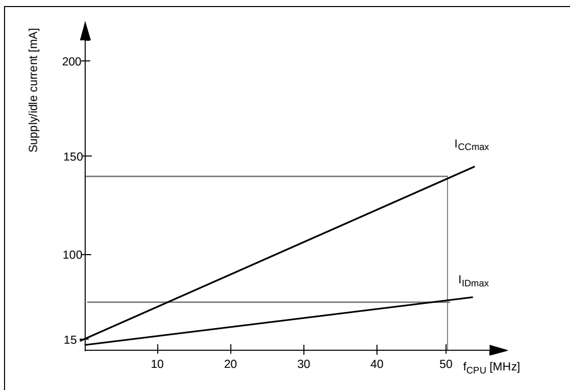
Figure 10 Supply/Idle current vs operating frequency
